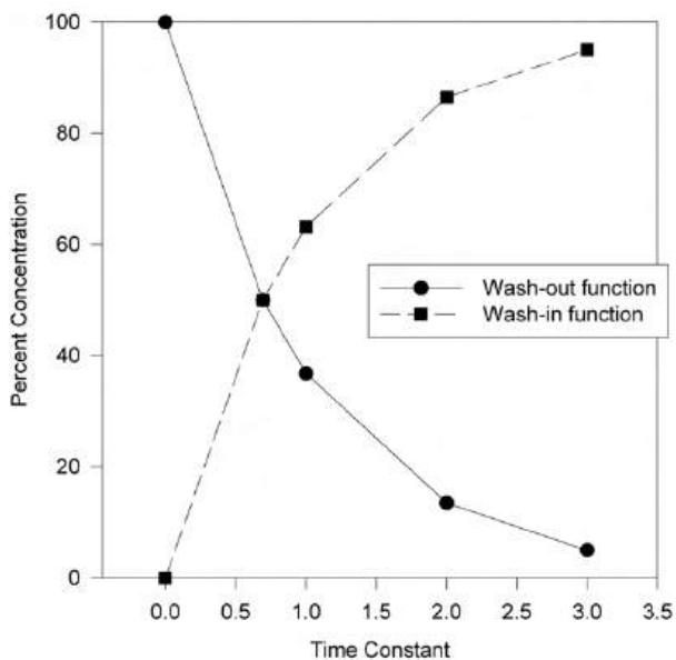
Figure 3 —Graphic representation of the wash-in and wash-out exponential functions, using a hypothetical example of a closed container, originally filled with gas A into which gas B is introduced. The wash-in and wash-out functions are used to determine the time constant for the enclosed volume or space. The gas concentration within the container can be readily determined from the time constant, which is calculated by dividing the container volume by the gas displacement rate. Figure taken from Meyer RE, Morrow WEM. Carbon dioxide for emergency on-farm euthanasia of swine. Journal of Swine Health and Production 2005;13(4):210–217, 2005. Reprinted with permission.
